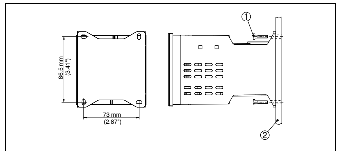
Fig. 8: Screw mounting
