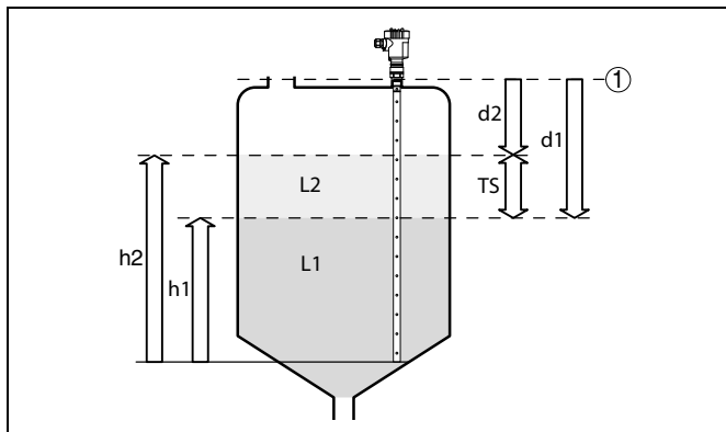
Fig. 3: Interface measurement
